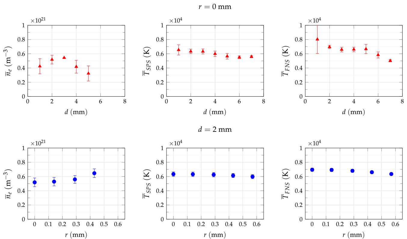
Figure 6. Average electron density ( \bar{n}_e ) and heavy particle temperatures ( \bar{T}_{SPS} , \bar{T}_{FNS} ) estimated on nozzle axis (first row of plots denoted with r = 0 mm) for different distances d downstream from nozzle outlet and for different lateral positions r at a distance d = 2 mm (second row of plots). In both cases, the experimental setup was triggered at peak current.
