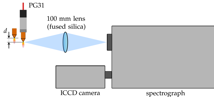
Figure 3. Schematic diagram of the spectroscopic experimental setup. The plasma generator PG31 is positioned perpendicularly to the vertically oriented entrance slit of the spectrograph on a micrometer table that allows the axial distance d from the nozzle outlet to be varied.
