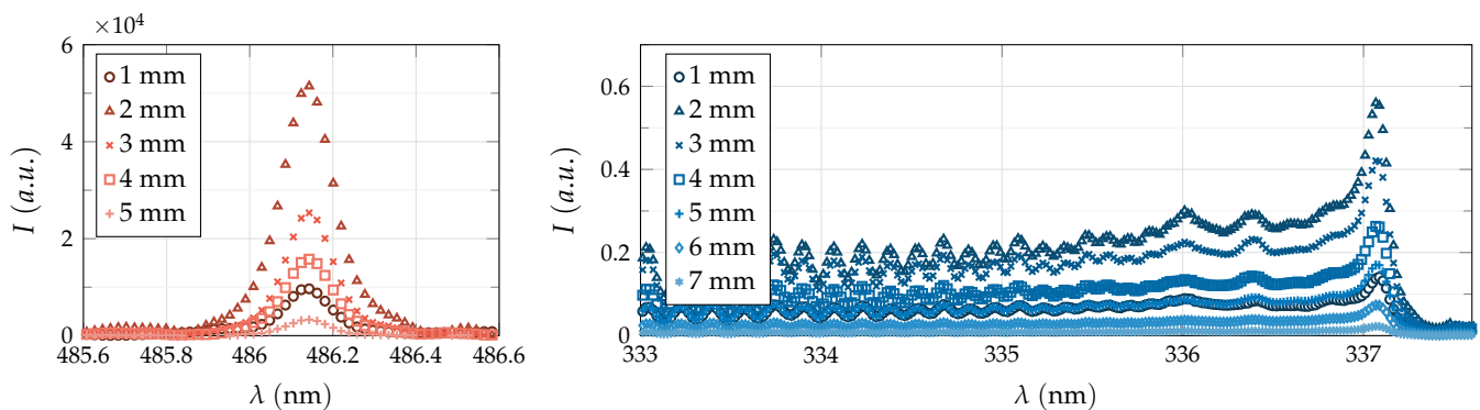
Figure 7. Experimental data used for estimation of n_e (left hand-side) and T_h (right hand-side). Due to imaging errors, a significantly lower intensity was recorded for a distance of 1 mm downstream from nozzle exit in both cases.
