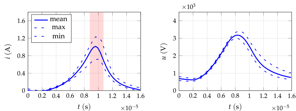
Figure 2. Typical voltage and current traces recorded prior to the power supply at an operating frequency of 60 kHz and a power setting of 100%. The trigger timeframe at which the experimental setup was triggered is marked in the current plot.
