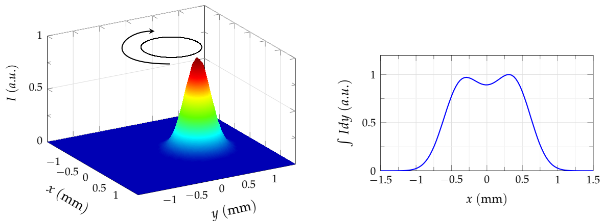
Figure 8. A two-dimensional Gaussian approximates the intensity emitted by the discharge channel. After integration on a detector, a bimodal intensity distribution can be observed when the movement of the channel is taken into account.
