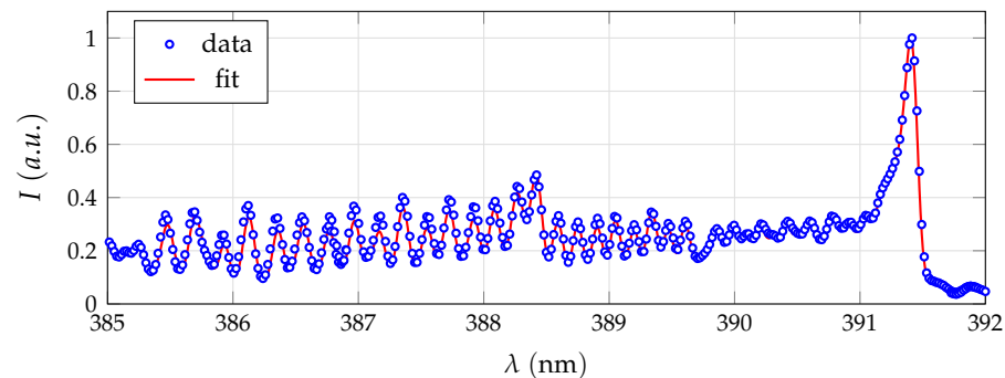
Figure 1. Rotational structure of a band sequence of the (0,0)-transition of the B^2\Sigma_u^+ \rightarrow X^2\Sigma_u^+ system of N_2^+ measured experimentally at peak current for the discharge operated at 60 kHz. Based on the calculated fit, a heavy particle temperature of 6300 K was estimated.
