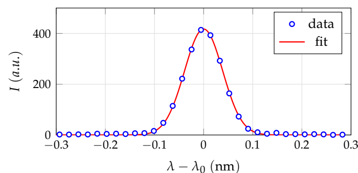
Figure 4. The instrumental profile of the spectroscopic setup determined by a Gaussian fit of a krypton emission line at \lambda_0 = 450.24 nm. The FWHM is 0.1 nm.
