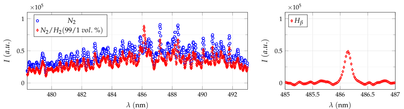
Figure 5. The left plot shows an N_2 and an N_2/H_2 spectrum after correction with the radiance calibration standard, recorded with similar camera settings at nozzle axis ( r = 0 mm) for an axial distance of d = 2 mm. The plasma generator was operated at 60 kHz and the experimental setup was triggered at peak current of \sim 1.0 A (power setting of 100%). The hydrogen \beta -line shown in the right plot is obtained after subtracting the pure nitrogen spectrum (multiplied by a variable scaling factor) from the hydrogen-containing measurement.
