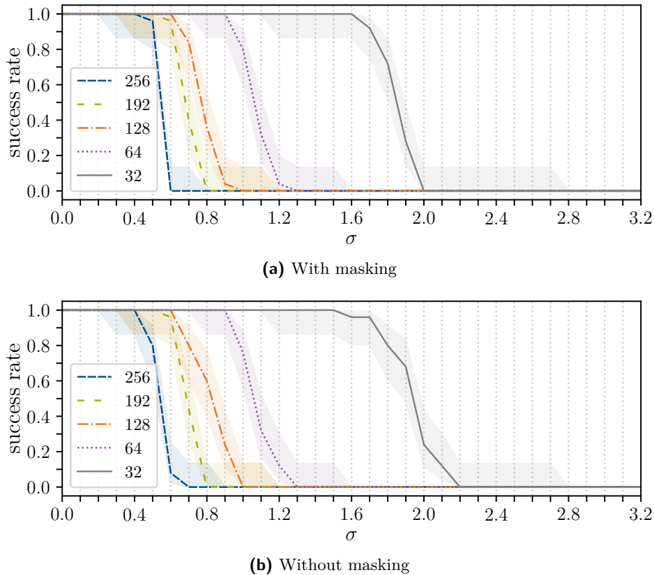
Figure 5.3: Attack results for different noise levels \sigma with non-zero coefficients in contiguous blocks. The figures show the attack success rate for the masked (a) and unmasked (b) implementations with the non-zero values in a contiguous block (see Figure 4.1). Each data point within the relevant area is the average of 25 runs with a step-size of 0.1 for \sigma . The shaded area marks the 95% confidence interval. In comparison to Figure 5.2, the noise tolerance is mainly decreased for a low number of non-zero coefficients (i.e. 64 and 32). Note, that the graph for 256 non-zero coefficients is identical to Figure 5.2, as this is the non-sparse case.
