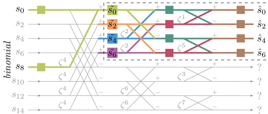
Figure 4.2: Recovering the private key from partial knowledge of \hat{s} . After inference of e.g. the upper half of \hat{s} , the original key can be recovered as follows. First note, that the last layers of the NTT can be reversed inside the upper half up to the intermediate polynomial \tilde{s} . From here, each coefficient can be independently brute forced by its original inputs, which are sampled from small binomial distributions, e.g. \{-2, \dots, 2\} . Here \tilde{s}_0 = s_0 + \zeta^4 s_8 which results in only 5^2 = 25 possible combinations.
