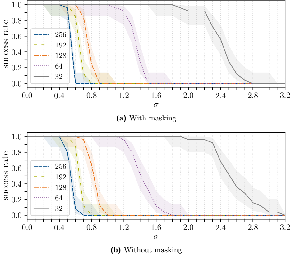
Figure 5.2: Attack results for different noise levels \sigma with distributed non-zero coefficients. The figures show the attack success rate for the masked (a) and unmasked (b) implementations, where the sparse vectors are generated with BKZ. Each data point within the relevant area is the average of 25 runs with a step-size of 0.1 for \sigma . The shaded area marks the 95% confidence interval. It can be seen that with a decreasing number of non-zero coefficients (given in the legend) the achievable noise tolerance is significantly increased.
