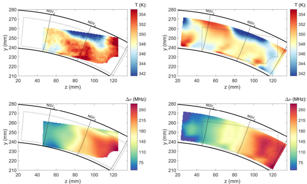
Fig. 3: Comparison of temperature (top) and Doppler shift (bottom) maps measured with FRS (left) and interpolated probe data (right). Black dashed lines mark respective areas covered by FRS and probe measurements, black solid lines mark the channel boundaries.
