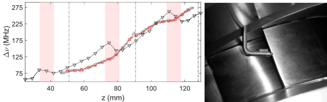
Fig. 4 left: Radial centreline profile of the Doppler frequency-shift for FSM-FRS (gray, \times ) and five-hole probe (black, \nabla ) measurement results. Red lines represent FSM-FRS results mapped onto the five-hole probe measurement grid. Dashed-dotted lines mark NGV trailing edge positions projected onto the measurement plane, red transparent areas indicate respective wake regions. Fig. 4 right: Dimension and arrangement of the five hole probe inside the flow channel.
