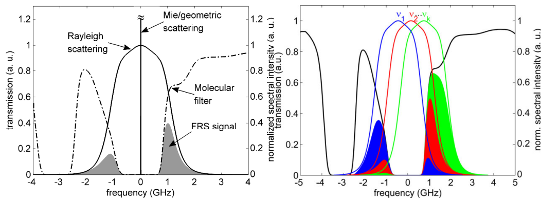
Fig. 1 left: Narrow linewidth laser light scattering is strongly attenuated by the molecular filter, while portions of Rayleigh scattering pass through. Fig. 1 right: Frequency scanning method: The laser's output frequency is modulated multiple times along the molecular filter's transmission profile.
