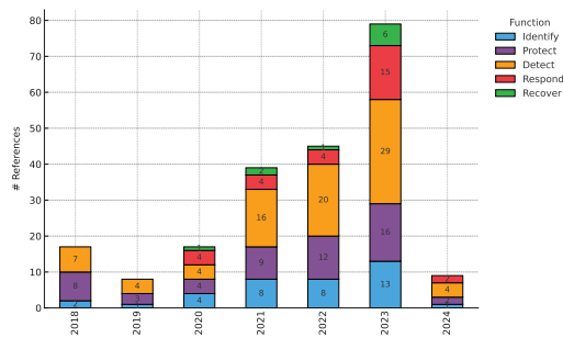
Fig. 7. NIST CSF function references (2018–2024), highlighting growth in response and recovery.
