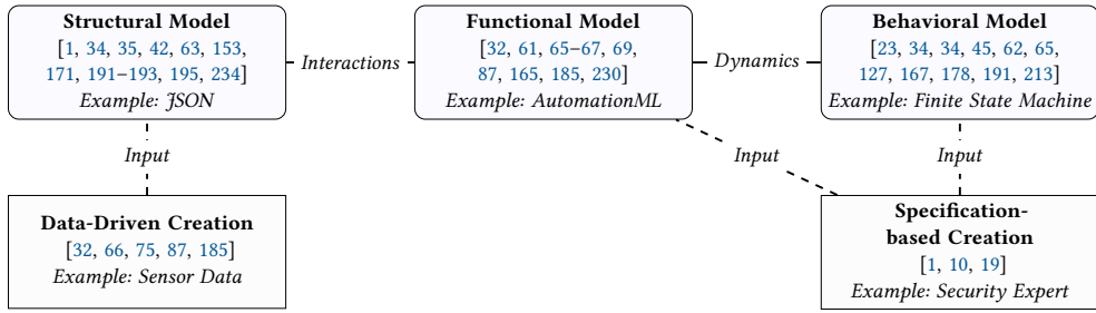
Fig. 6. Illustration of structural, functional, and behavioral models in digital twin research.
