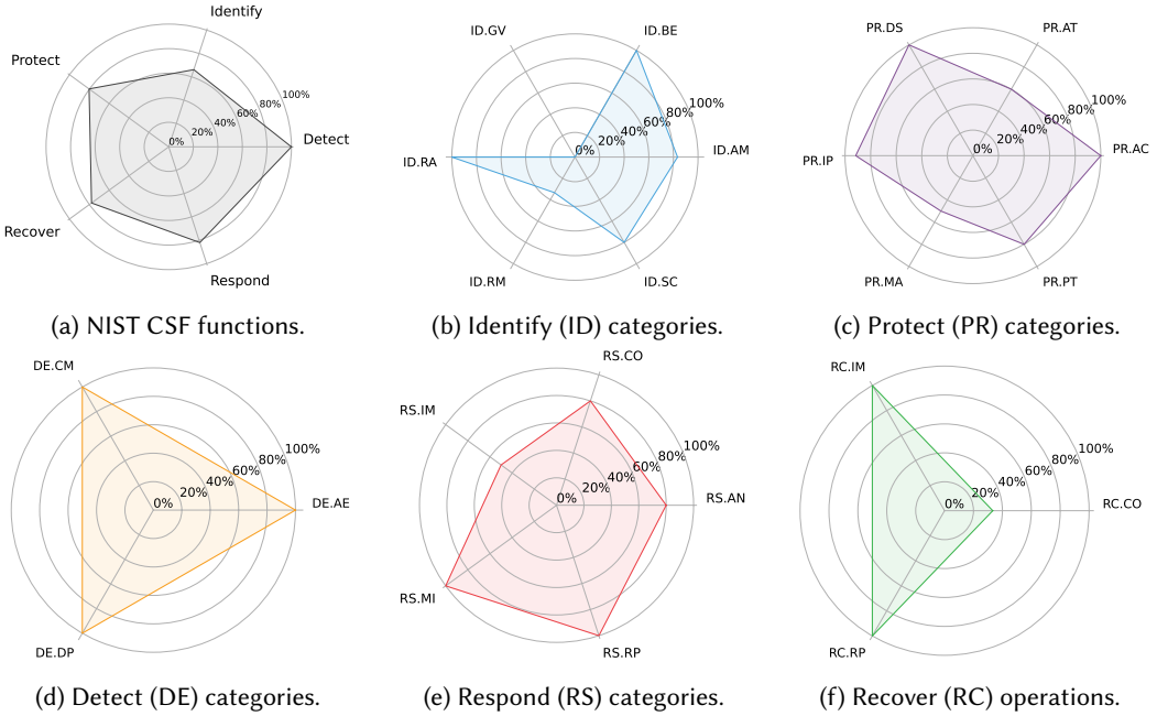
Fig. 5. Digital twins in relation to the NIST Cybersecurity Framework (CSF) if they have been addressed at least once. Digital twins' security operations were coded and manually mapped to the corresponding NIST CSF functions and categories.
