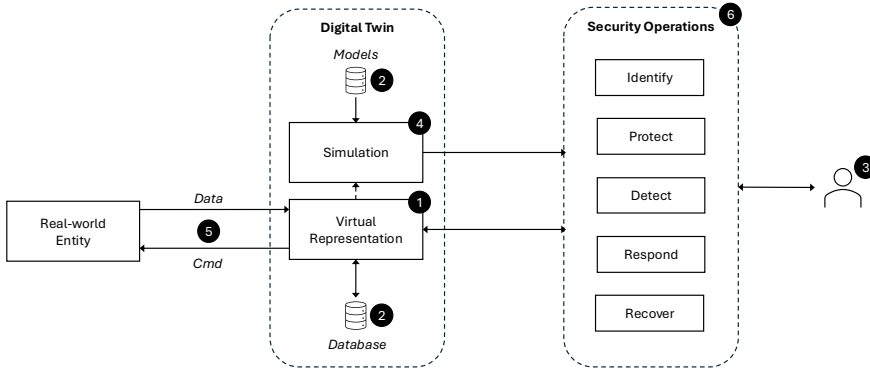
Fig. 4. Functional components of digital twins for security operations and their dependencies.
