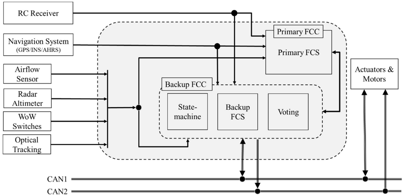
Fig. 2 Architecture of the Flight Control Computer
