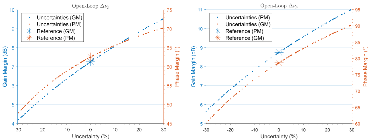
Fig. 9 Open-Loop Gain and Phase Margin with Uncertainties - left: Hover, right: Wingborne
