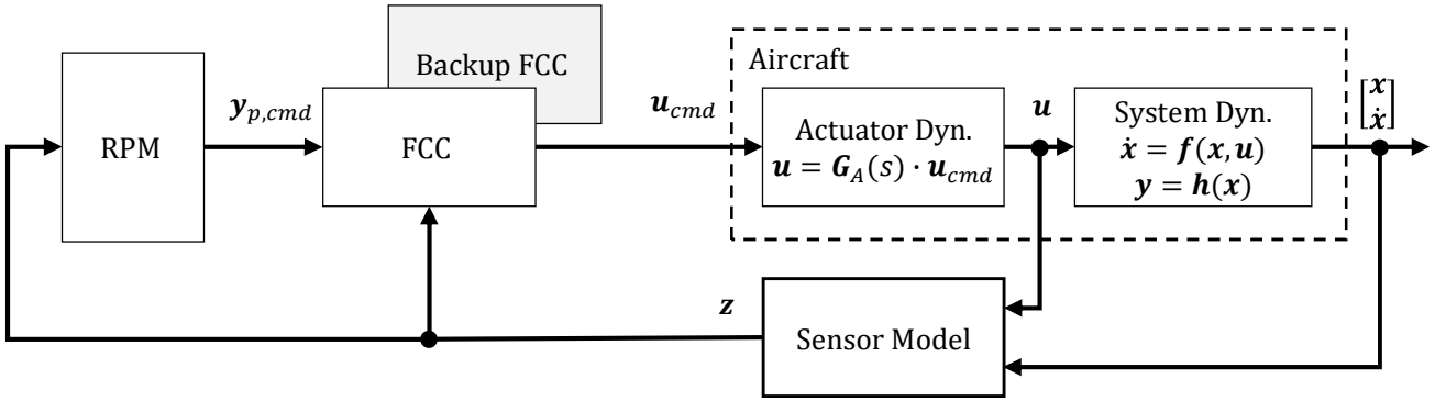
Fig. 8 System Simulation
