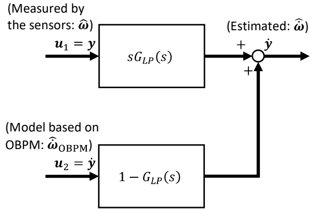
Fig. 7 Complementary Filter of the Angular Acceleration
