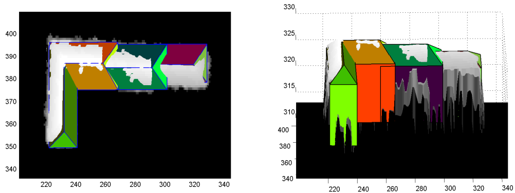
(a) Model superimposed on LP data – top view
