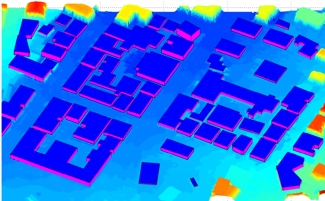
(b) 3D prismatic model put on top of DTM creates the LOD1 representation
