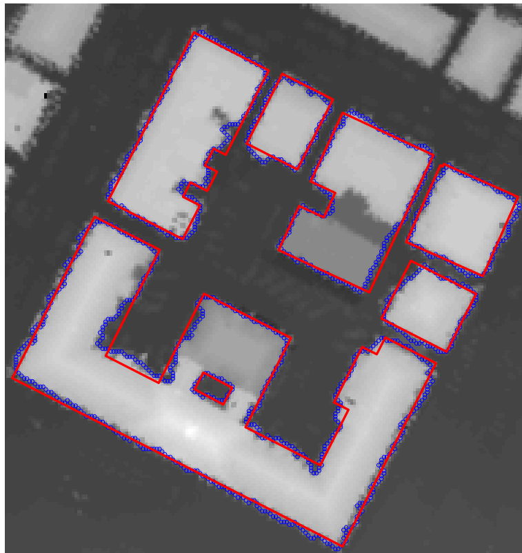
Figure 7.15: Building outline approximation result ( red polygons ) as well as the original extracted building boundaries ( blue polygons ) superimposed on LP image
