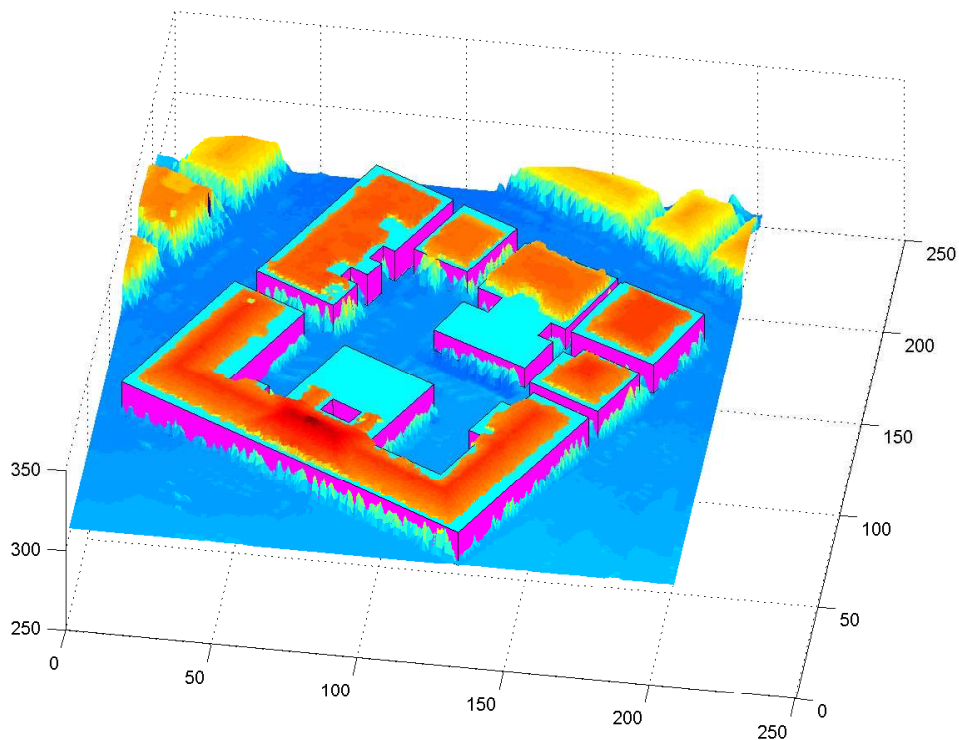
Figure 7.17: 3D prismatic models combined with surface model
