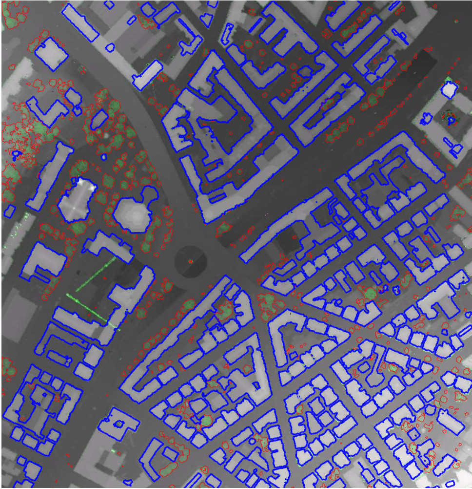
Figure 7.11: Classified building ( blue polygons ) and vegetation ( red polygons ) regions are superimposed on the gray scale LIDAR image that the pixels belonging to the vegetation index are colored by green.
