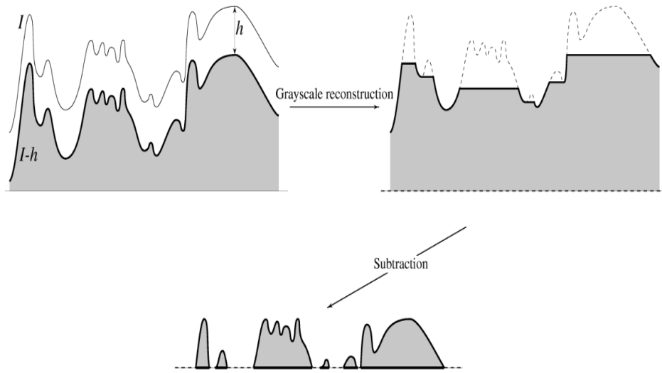
Figure 4.8: Reconstruction by geodesic dilation of a 1D mask signal I from a marker signal J . The marker signal is produced by subtraction of a constant offset h from the mask. The result of grayscale reconstruction using geodesic dilation is shown in the top right part. The subtraction of the reconstructed signal from the mask signal leads to the result given on the bottom (VINCENT, 1993)
