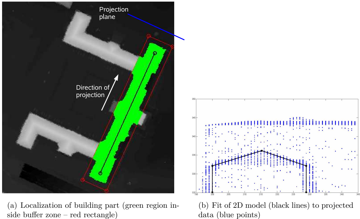
Figure 6.7: Projection-based modeling
