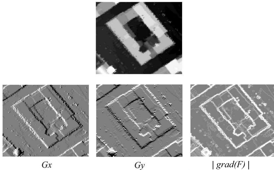
Figure 2.4: Gradient images
