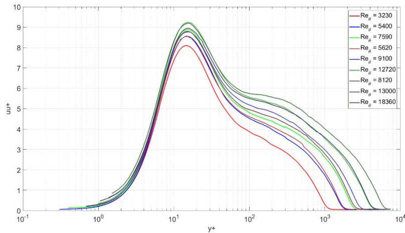
Figure 4: Streamwise Reynolds stress profiles in inner variable \overline{u'u'} = f(y^+) .
