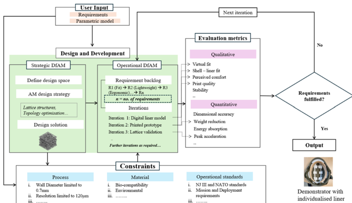
Figure 3. Structured iterative DfAM process showing information flow and feedback between user input, constraints, design, development, and evaluation
